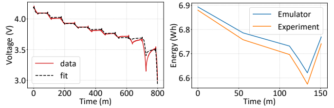
(a) Modeled battery emulator of LCO (b) Emulating MixMax versus real cylindrical batteries experiment.
