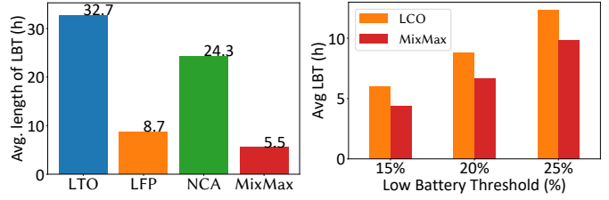
(a) Different battery types.
