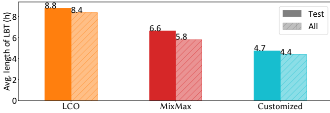
(a) Low battery time (LBT) results over a week.
