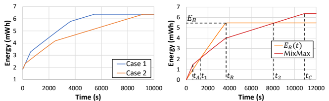
(a) Charging MixMax with two different energy distributions under the same total remaining energy. (b) Multi-stage charging speed of MixMax, compared with the charging speed of a single B-type battery.
