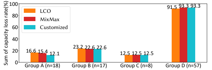
Fig. 18. Group-wise total aging evaluation of LCO, original MixMax, and customized MixMax.
